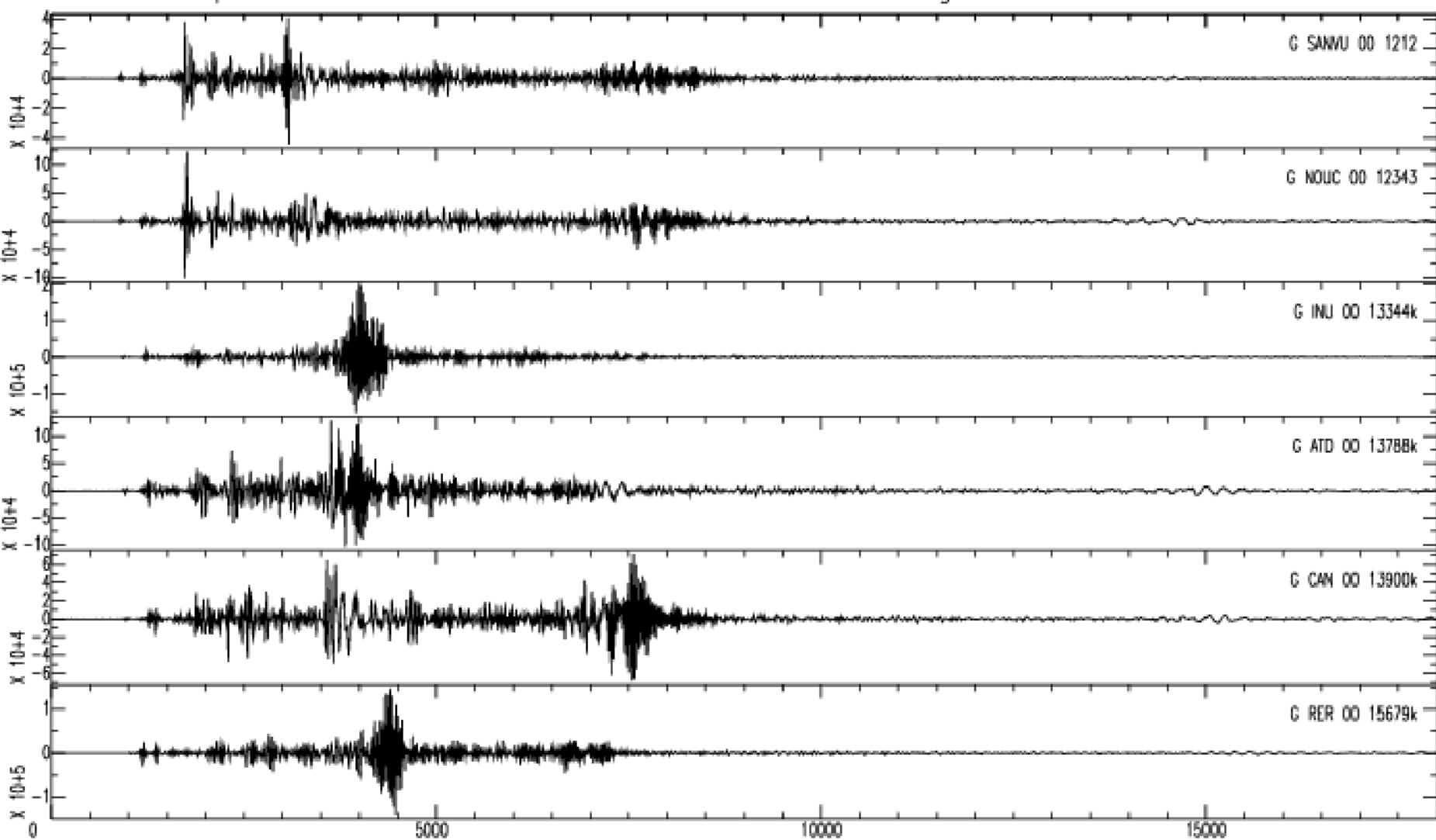
GEOSCOPE Stations/VHZ channel - Time in seconds - 0.002Hz high pass filtered data
