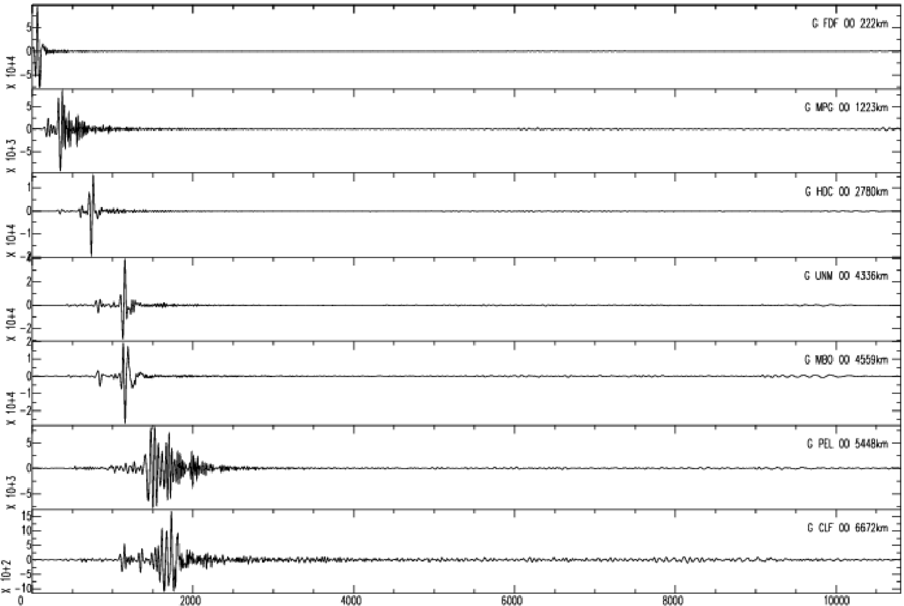
GEOSCOPE stations/LHZ channel - Time in seconds - data filtered between 0.003Hz and 0.02Hz
